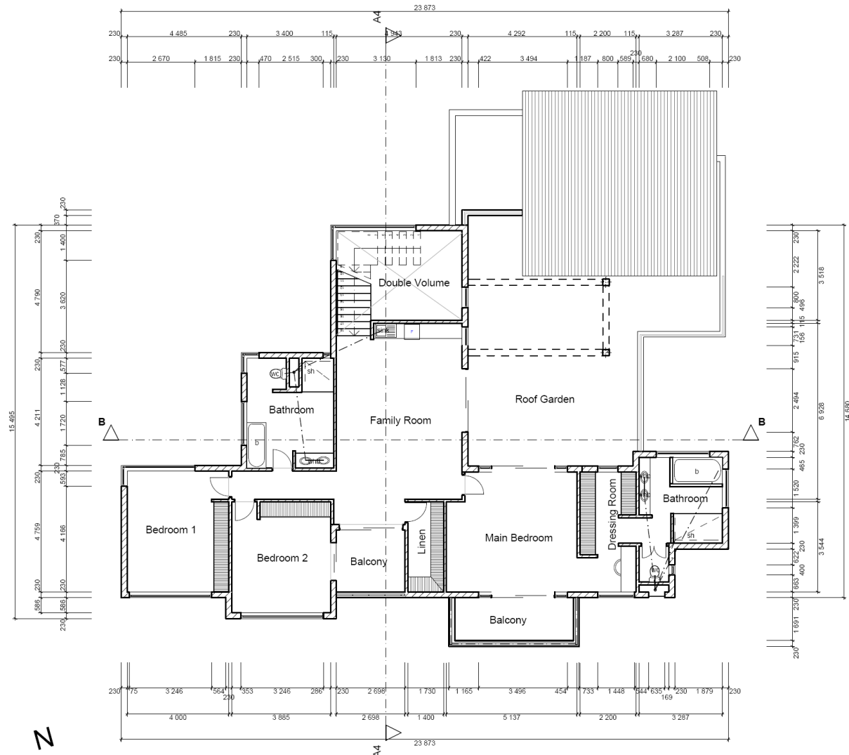
First Floor Plan Scale 1:100 (165m²)
